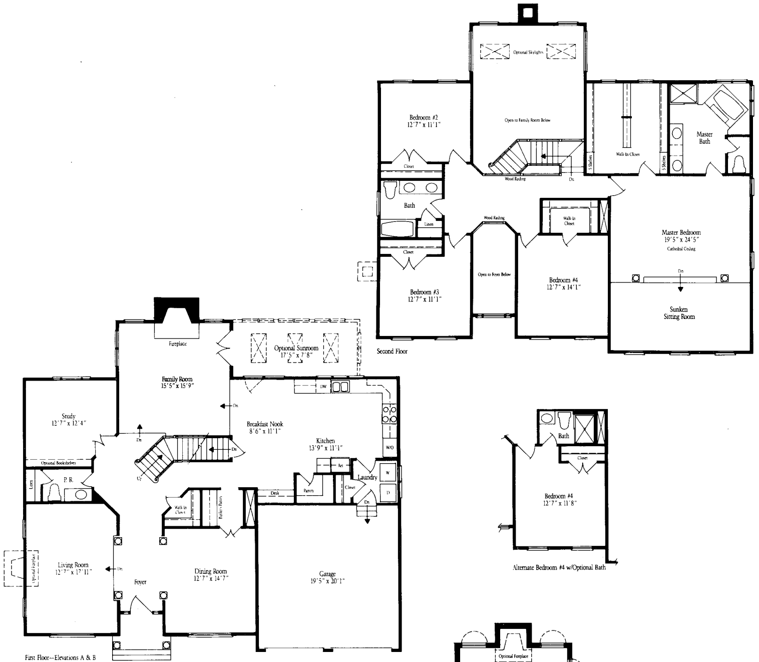
First Floor--Elevations A & B
